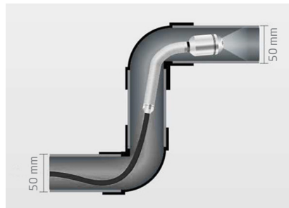
Pass through two 90° pipeline corner
